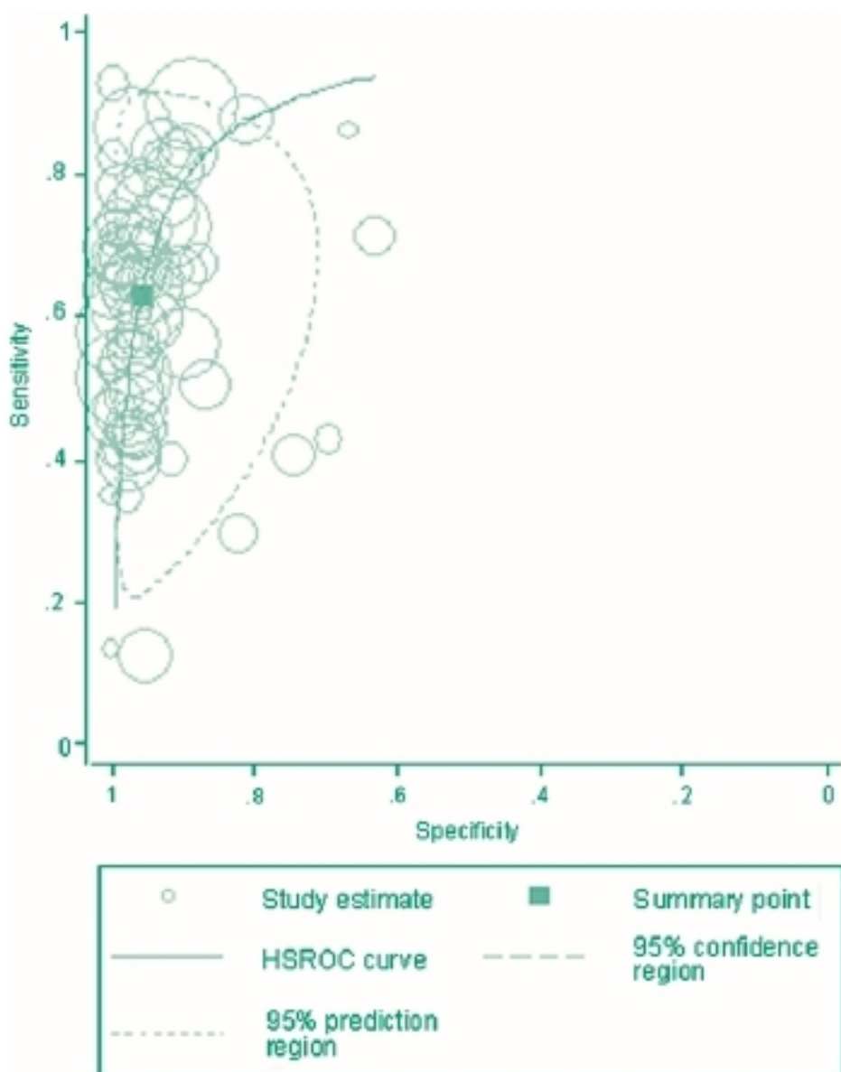
Figure. SROC plot of case-control and cohort studies combined.
