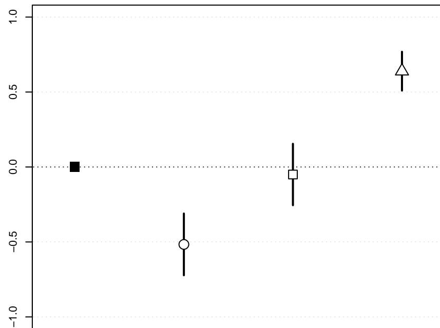
Calibration-in-the-large
