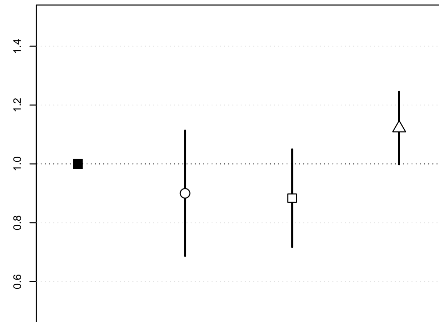
Calibration slope
