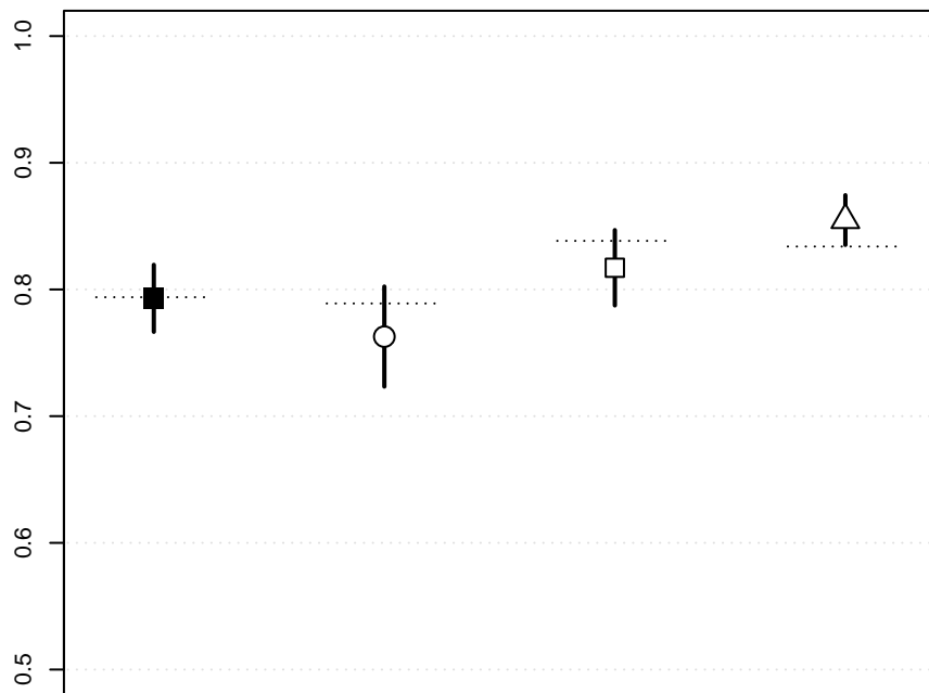
c-statistic
