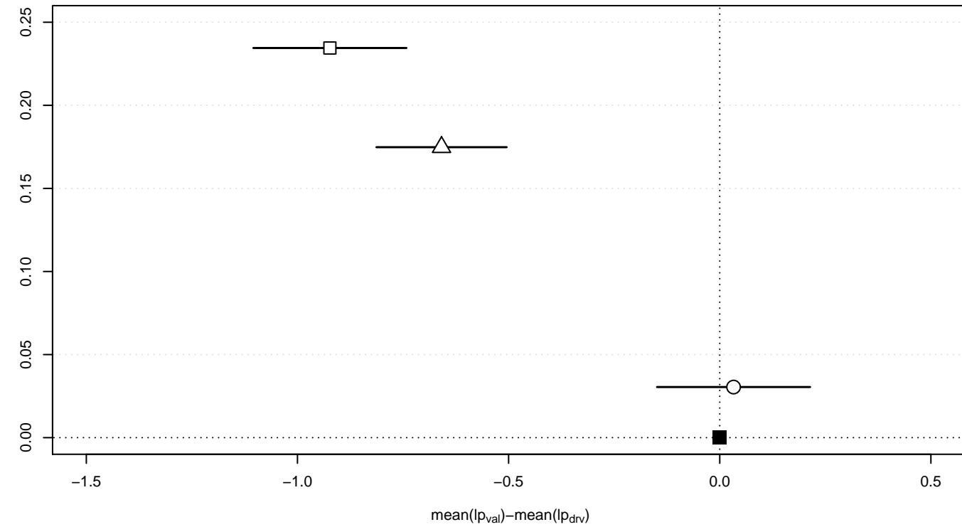
Calibration-in-the-large
